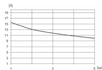
0501: l/h 1 bar 5 Pump head mod. I
