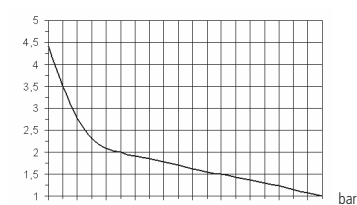
2001: 01 l/h bar 20 Pump head mod. I
