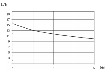
0510: l/h 10 bar 5 Pump body mod. K
