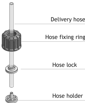
Fig. 5. Delivery hose / pump body assembly
