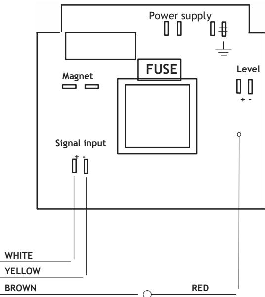
Fig. 39. VMS MF circuit diagram for connection to a pulse water meter with Hall effect
