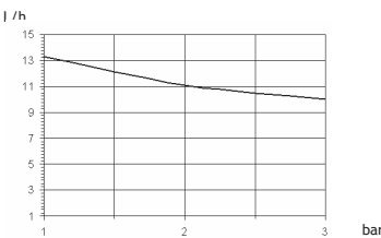
0310: l/h 10 bar 3 Pump body mod. K
