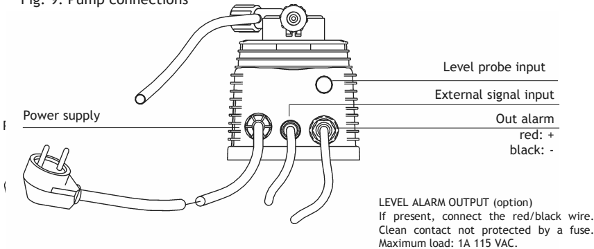
Fig. 9. Pump connections
