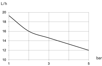
0512: l/h 12 bar 5 Pump body mod. K
