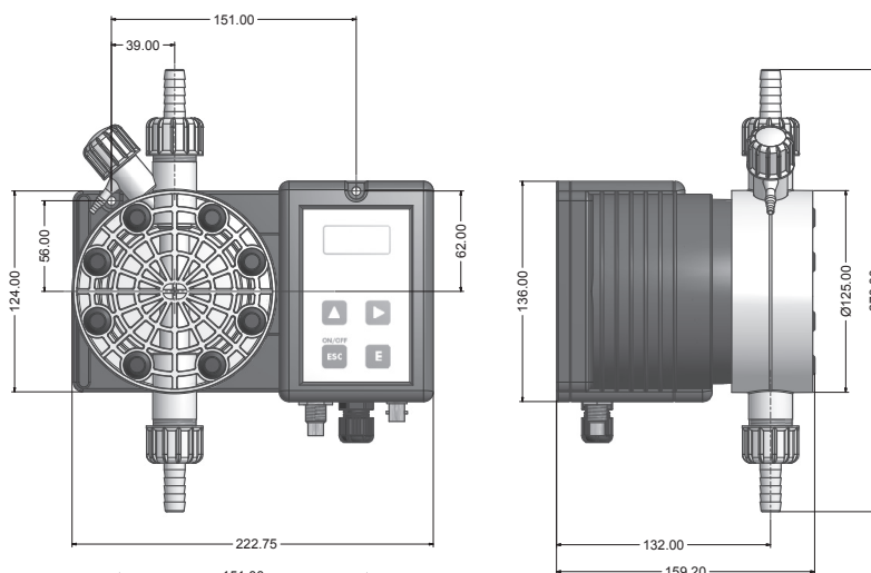
"N" - "P" PUMP HEAD
