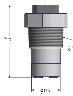
ECDIM/1
